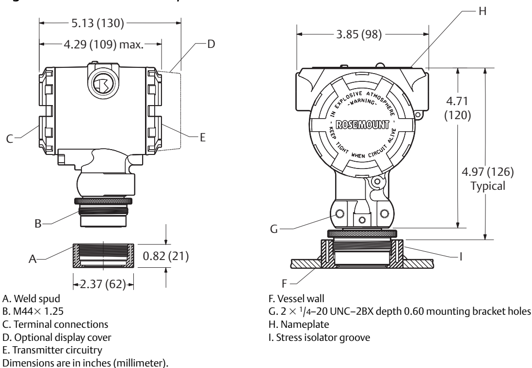
Figure 2. Rosemount 2090P 1½-in. Flush Mount
