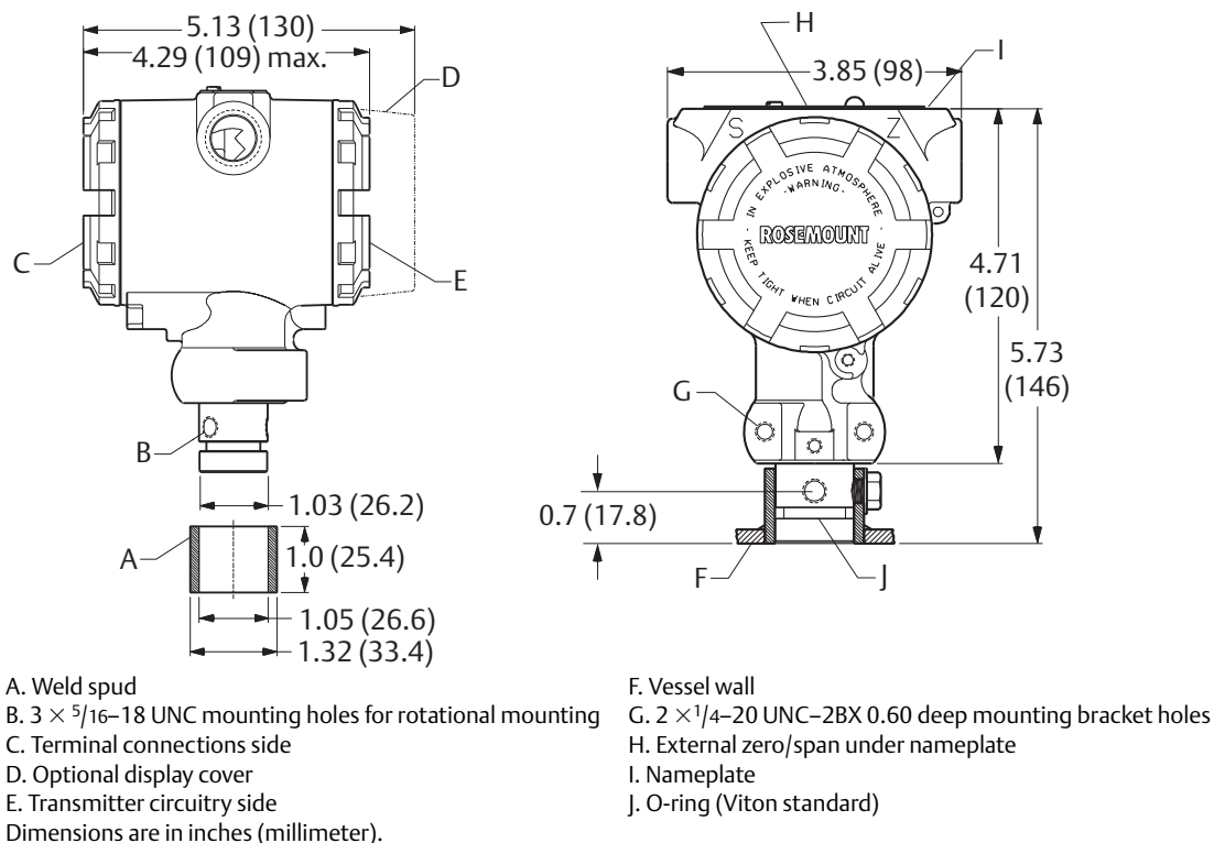
Figure 1. Rosemount 2090P 1-in. Flush Mount
