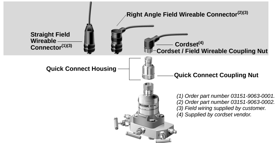
Figure 2-11. Rosemount 3051S Quick Connect Exploded View
