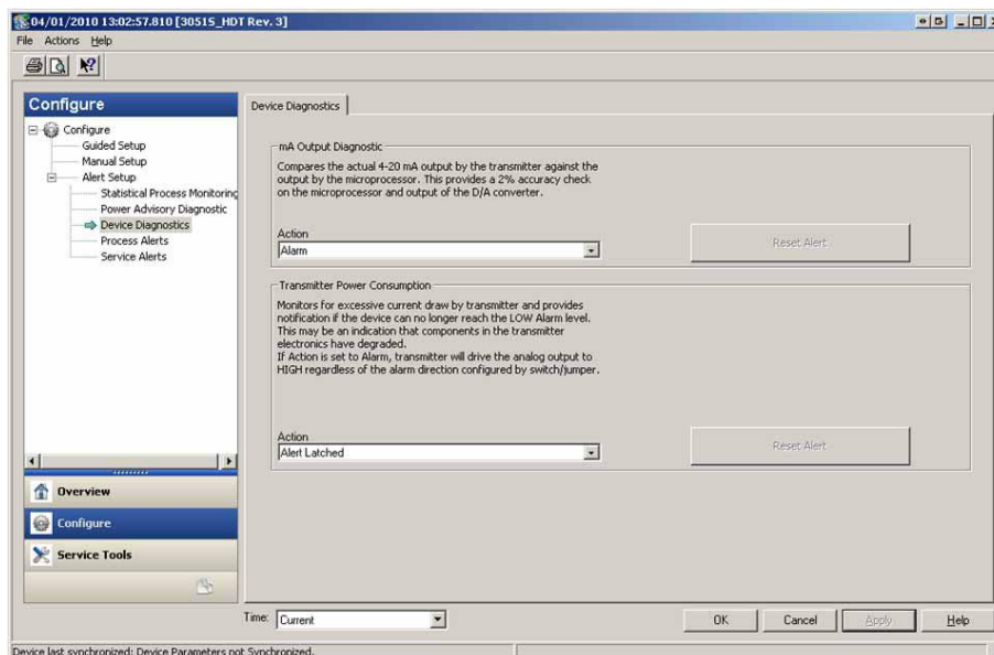
Figure 7-26. Device Diagnostics screen
