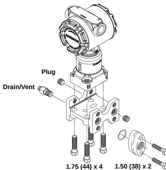
GAGE/ABSOLUTE TRANSMITTER
