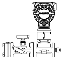
304 TRADITIONAL
