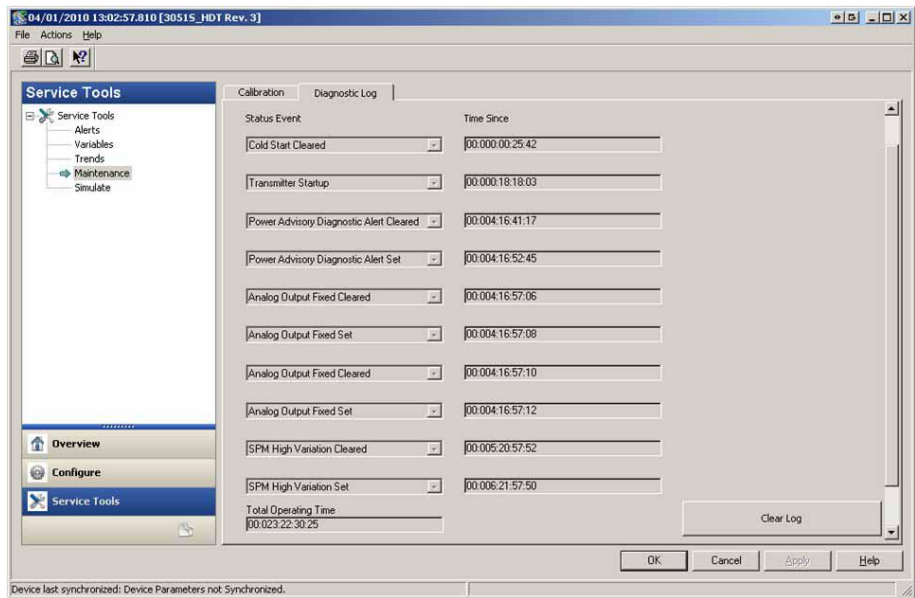
Figure 7-20 shows the Diagnostic Log screen where a set of ten events and time stamp can be seen.
