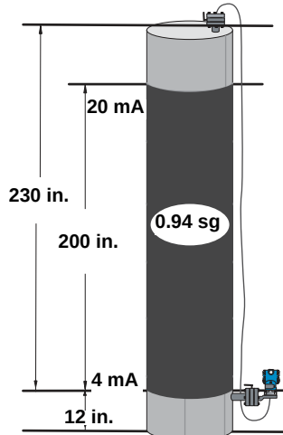
Figure 3-9. Example tank
