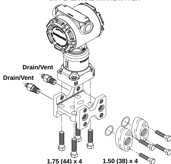
DIFFERENTIAL TRANSMITTER
