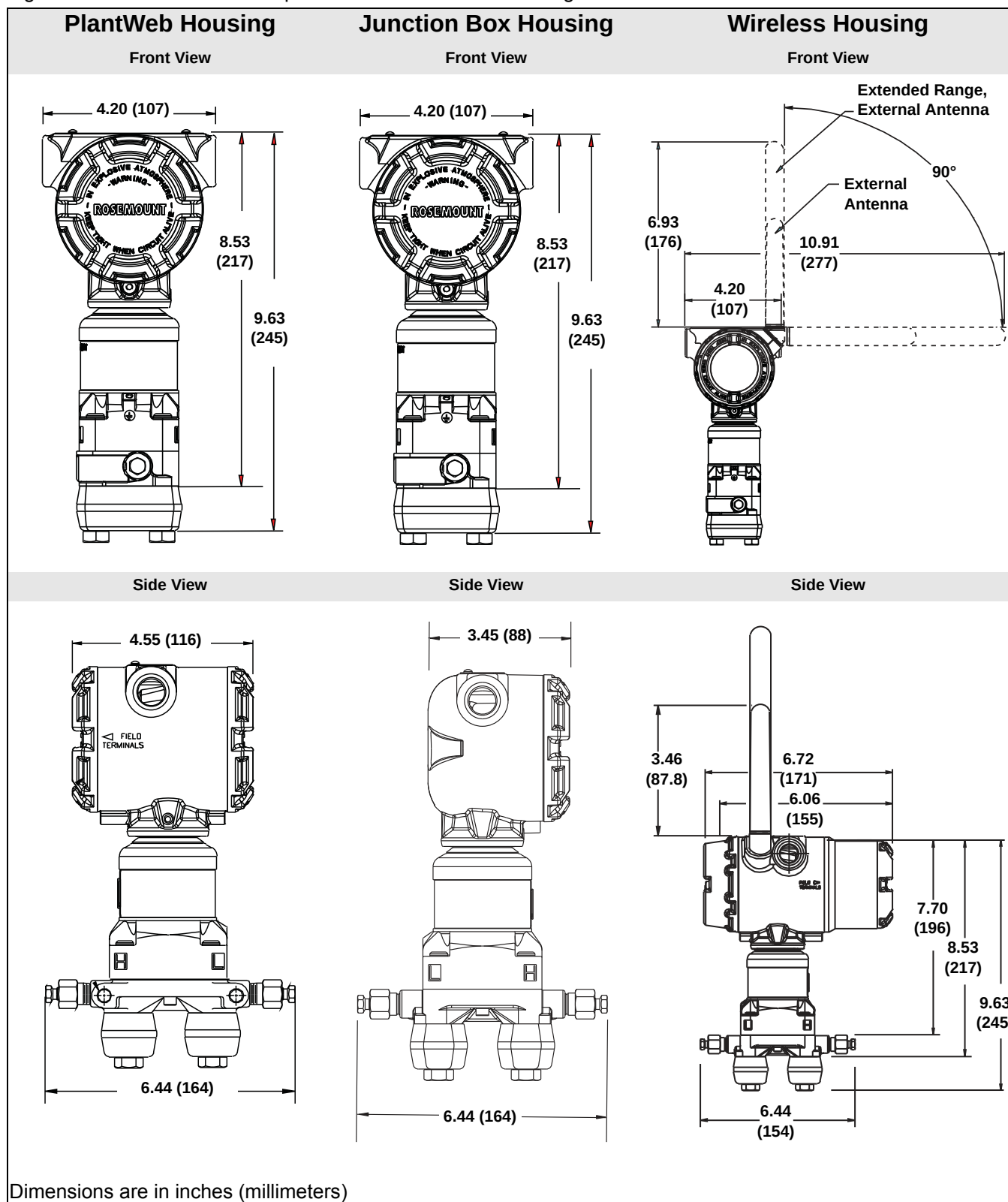
Figure A-1. Transmitter with Coplanar Sensor Module and Flange
