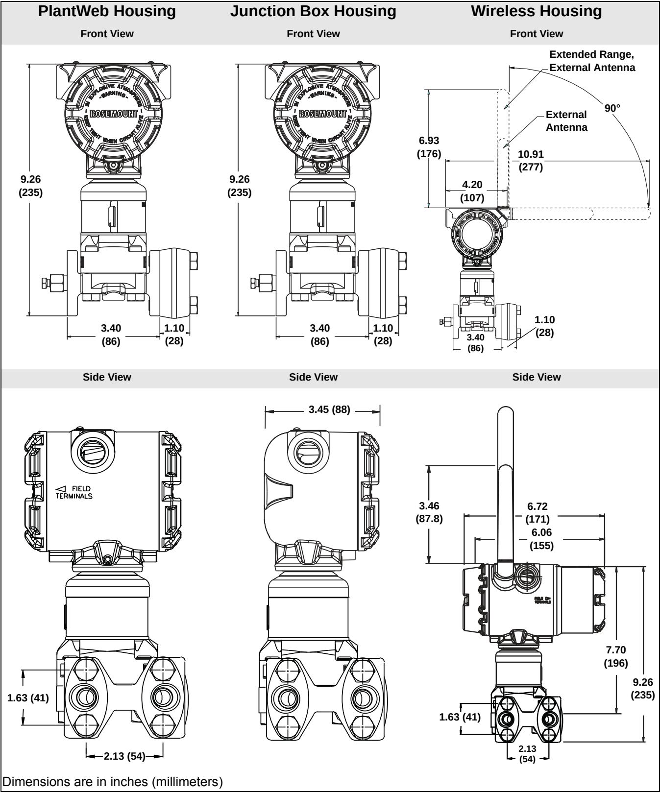
Figure A-2. Transmitter with Coplanar Sensor Module and Traditional Flange
