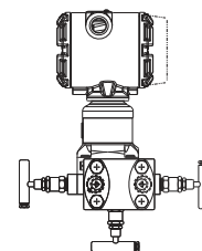
305 INTEGRAL TRADITIONAL
