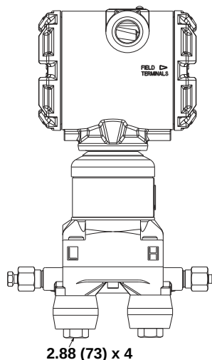
Transmitter with Flange Adapters and Flange/ Adapter Bolts
